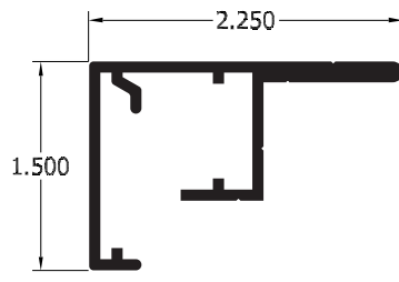
Flat 1 1/2" Retainer Part #2052
