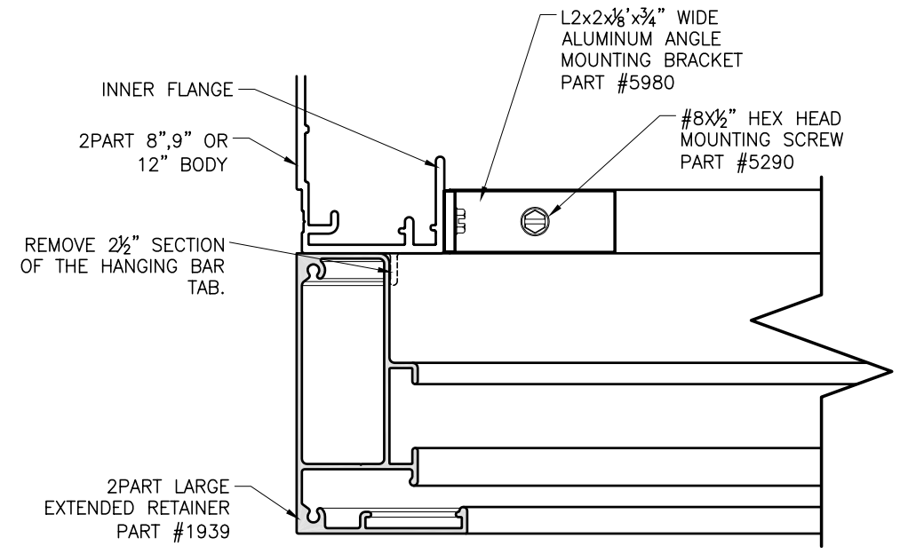
TOP VIEW SECTION SCALE : 1/2"=1"
