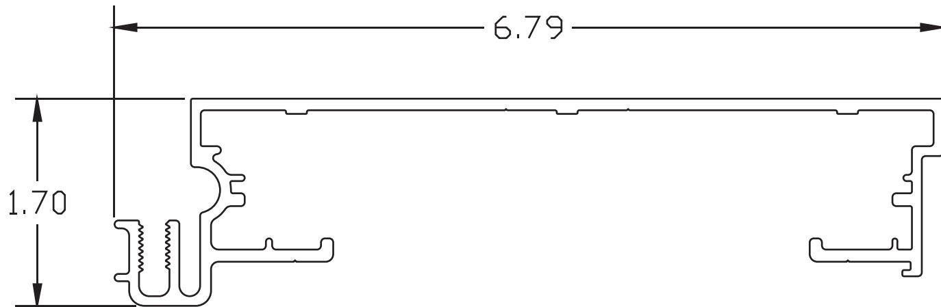
SINGLE FACE BODY #2025 SCALE : FULL SIZE
