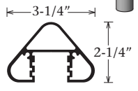
Triangular Post w/Radius Edges *Part #1250
