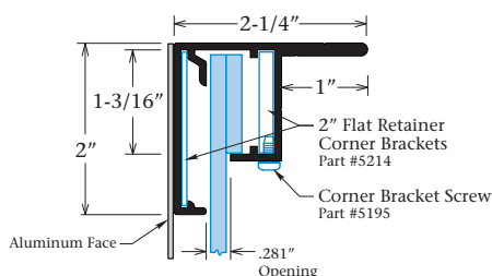
Flat 2" Retainer Part #2047
