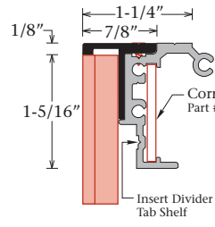
Insert End Cover Part #1696 Access Frame Part #1690
