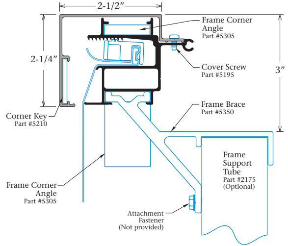
Dual Frame Part #2065 2-1/4" Dual Frame Cover Part #2075
