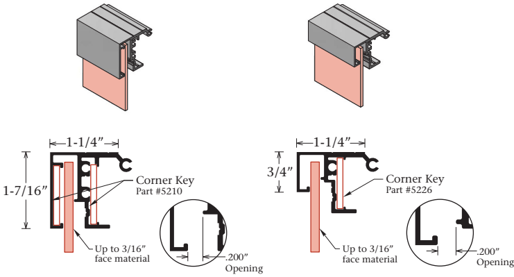
Slide Retainer Part #1624
