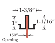
1/8" Panel Adaptor Part #1203
