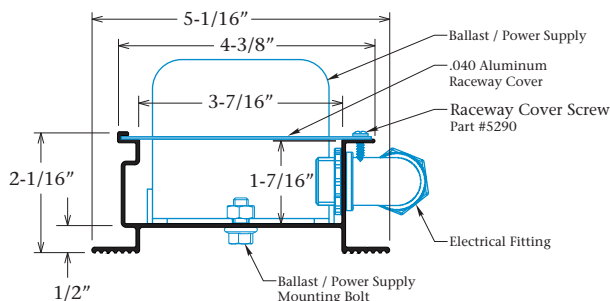
Ballast Raceway Part #1969
