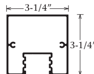
Square Post Part #1233
