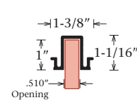
1/2" Panel Adaptor Part #1204
