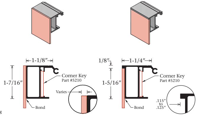
Frameless Retainer Part #1631
