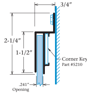
1.5" Z-Molding Part #1947
