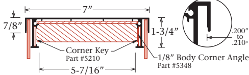
Slide Body Part #1560 For Removable Faces
