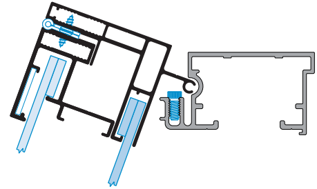
2Part Large Outer Frame Part #1941
