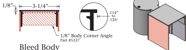
Bleed Body Part #1270 For Fixed Faces
