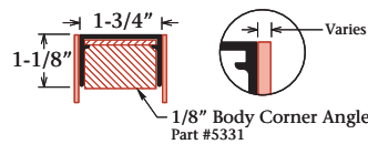
Frameless Body Part #1125 For Fixed Flush Faces
