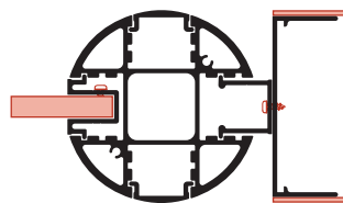
One Reveal Position 0"
