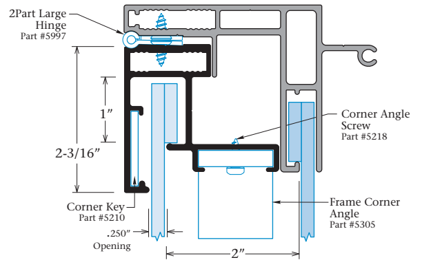
Large Inner Frame Retainer Part #2097
