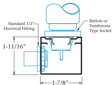
Large Socket Raceway Part #1983 Socket Raceway Cover Part #1987
