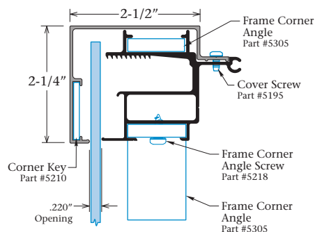
2-1/4" Dual Frame Cover Part #2075
