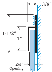
1" H-Molding Part #1945
