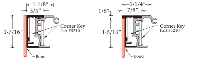
Frameless Cover Part #1693 Access Frame Part #1690
