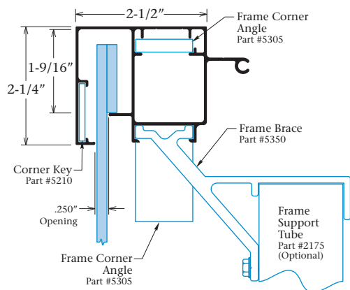
2-1/4" Retainer Part #2045
