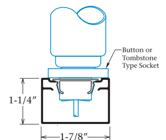
Socket Raceway II Part #1985 Socket Raceway Cover Part #1987
