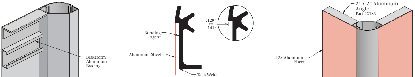
2" Radius Edge Part #1880
