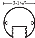
Round Post Part #1237
