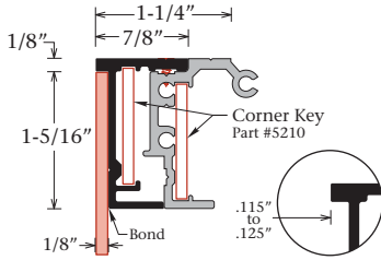
Bleed Cover Part #1692 Access Frame Part #1690
