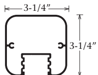
Square Post w/Radius Edges Part #1235
