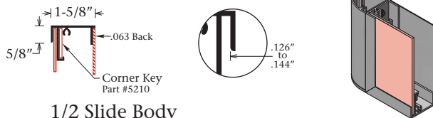
1/2 Slide Body Part #1265 For Removable Faces
