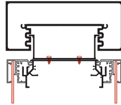
Three Reveal Positions 0", 1/2" & 1"
