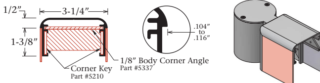
1/4 Round Body Part #1280 For Fixed Faces
