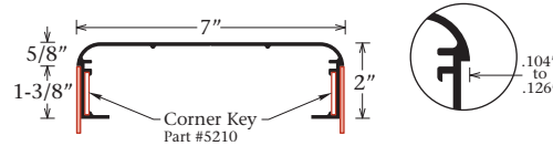
1/4 Round Body *Part #1580 For Fixed Faces
