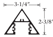
Triangular Post Part #1240
