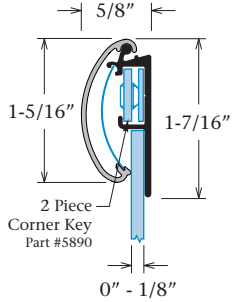
Snap Frame Part #1899 Snap Frame Radius Cover Part #1896
