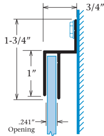
1" Z-Molding Part #1946
