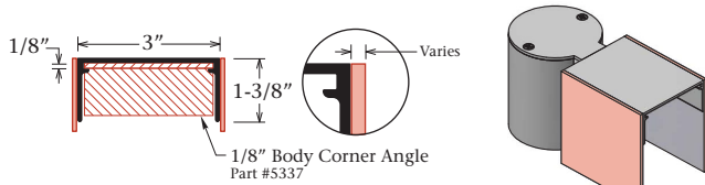
Frameless Body Part #1275 For Fixed Flush Faces
