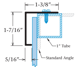
1-3/8" L-Molding Part #1943
