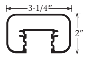
Rectangular Post w/ Radius Edges Part #1230
