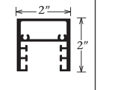
*Square Post Part #1110
