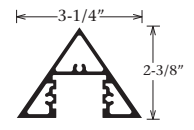
Triangular Post Part #1240
