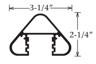
Triangular Post w/ Radius Edges Part #1250
