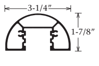
*Radius Post Part #1210
