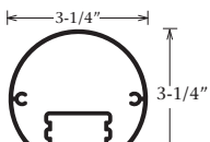
Round Post Part #1237
