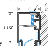
Wall Mount Tension Square Cover Part #2088
