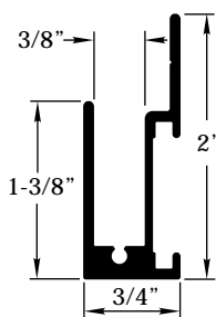
1-3/8" Wall Frame Part #1949
