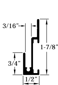
3/4" Wall Frame Part #1948
