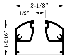
Edge Lit LED 1/4 Round Part #1996
